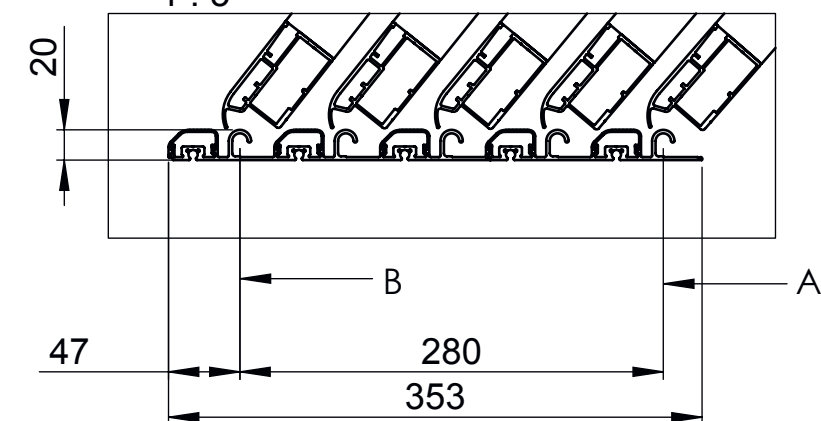
DETAIL A 1:5
